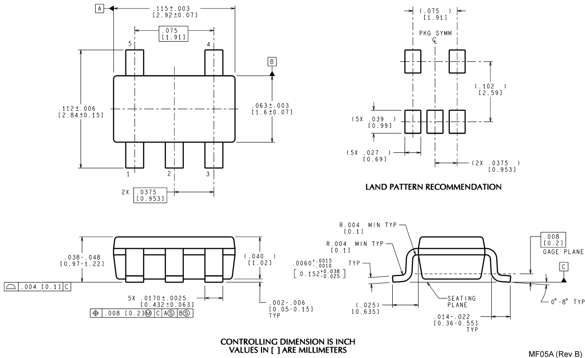
5-Lead Small Outline Package (M5) NS Package Number MF05A
