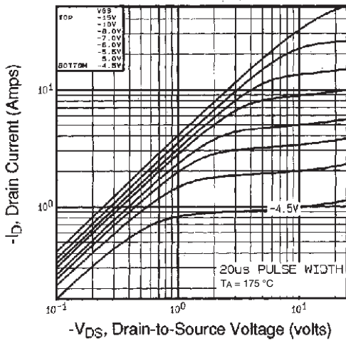
Fig. 2 - Typical Output Characteristics, T_A = 175\text{ °C}
