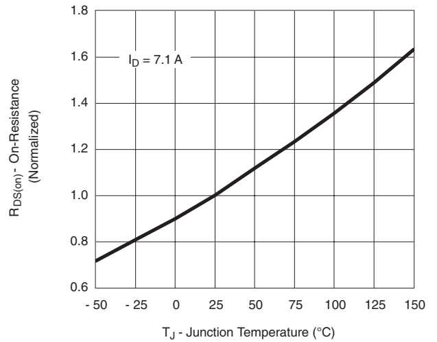
I_D = 7.1 A On-Resistance vs. Junction Temperature
