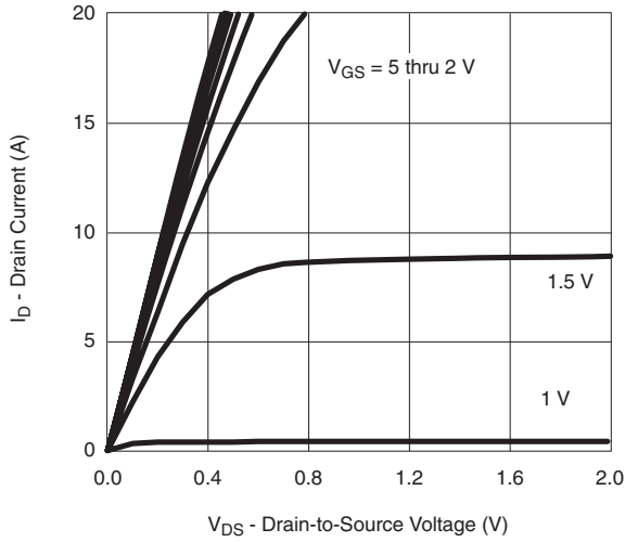
V_{GS} = 5 thru 2 V Output Characteristics
