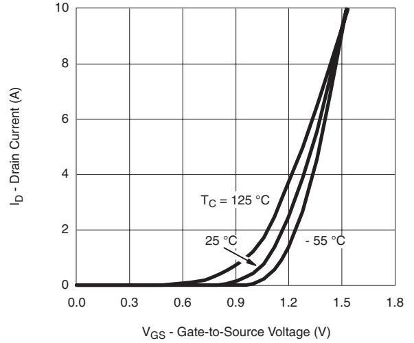
T_C = 125 °C 25 °C -55 °C Transfer Characteristics
