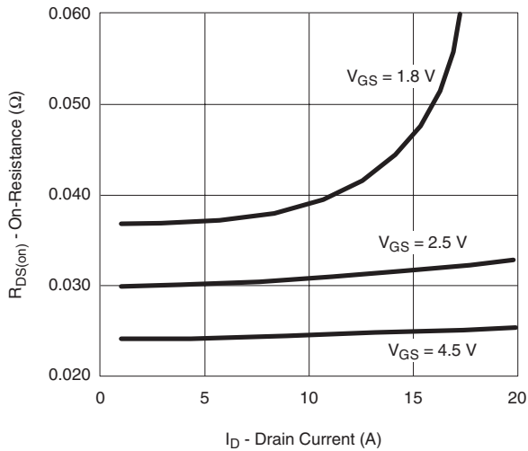
V_{GS} = 1.8 V V_{GS} = 2.5 V V_{GS} = 4.5 V On-Resistance vs. Drain Current and Gate Voltage
