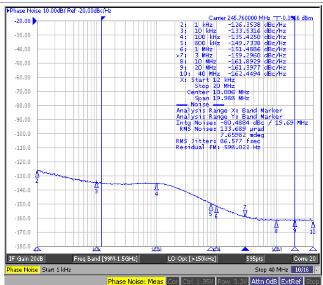
Figure 26. DCLKout2, 245.76 MHz LVPECL20 w/ 240 \Omega emitter resistors DCLKout2_3_IDL = 1, DCLKout2_3_ODL = 1
