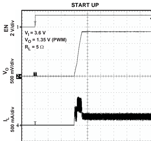
t – Time = 50 \mu s/div Figure 43.
