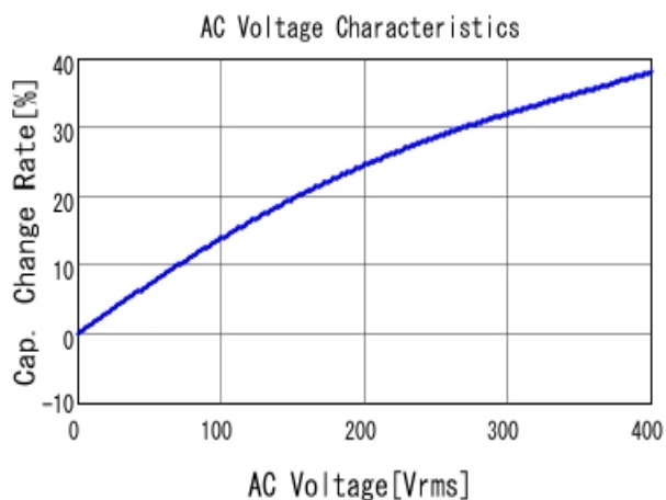
■ DE2B3SA471KA3BY02F C-AC Voltage capchange, DCOV, 20.0
