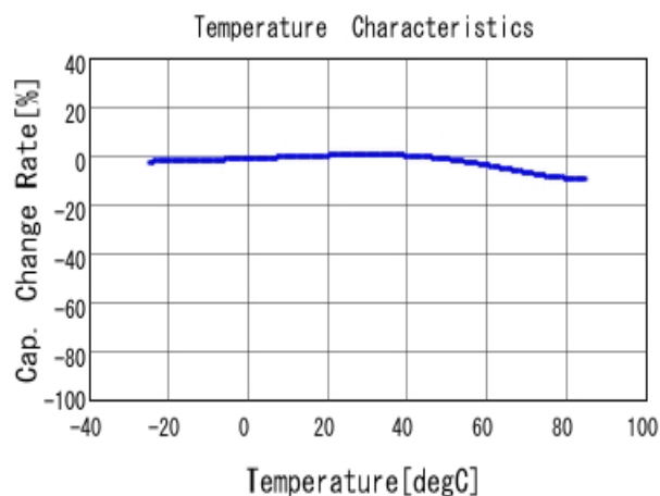
■ DE2B3SA471KA3BY02F C-Temp. capchange, DCOV, AC1Vrms
