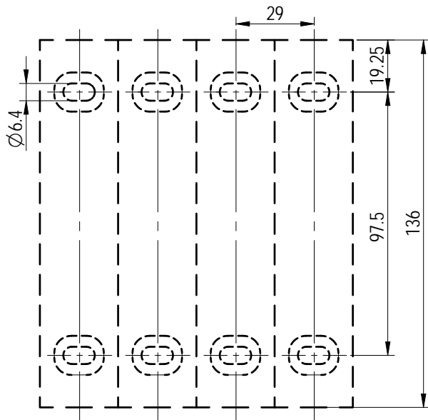
面板安装示意图/Panel installation diagram
