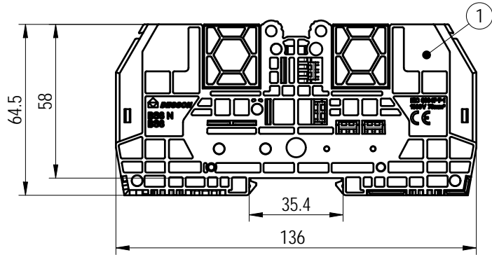
面板安装示意图/Panel installation diagram
