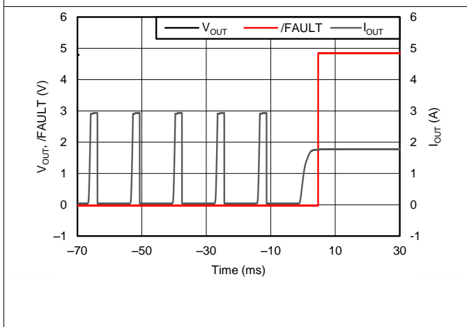
Figure 27. Output Short to 2.5-Ω Load Recovery Response
