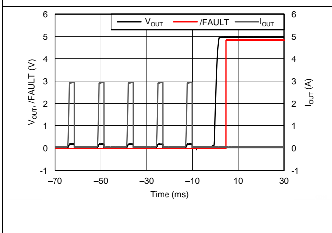
Figure 29. Output Short to No Load Recovery Response
