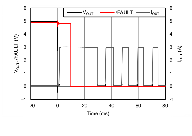
Figure 28. No Load to Output Short Transient Response
