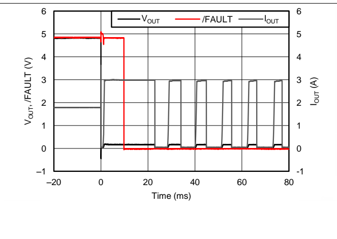
Figure 26. 2.5 Ω to Output Short Transient Response
