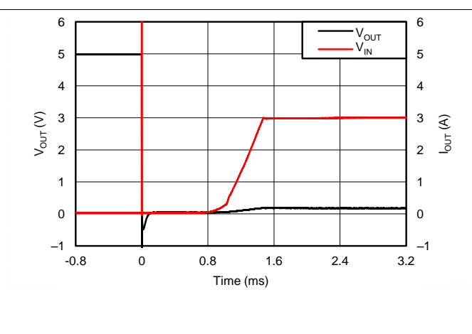
Figure 30. Hot-Short With 50 mΩ
