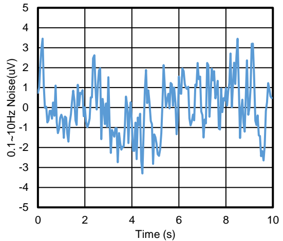
Figure 20 0.1 to 10 Hz Voltage Noise, V_{CM} = 4\text{ V}
