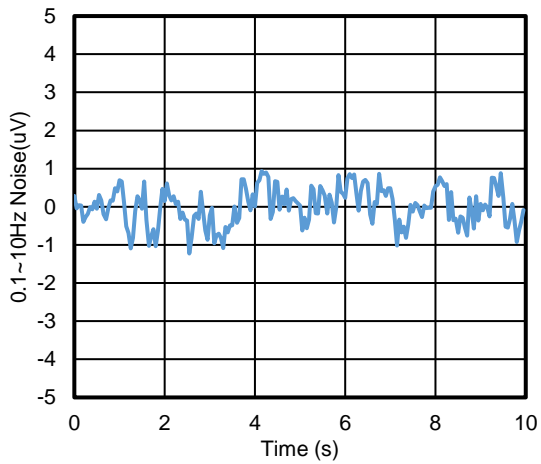
Figure 19 0.1 to 10 Hz Voltage Noise, V_{CM} = 1\text{ V}
