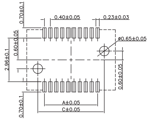
PCB LAYOUT
