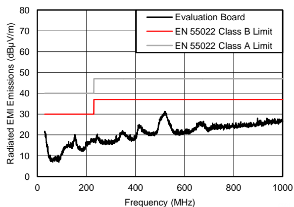
Radiated Emission Graph V_{IN} = 24 V, V_{OUT} = 3.3 V, F_S = 500 kHz, I_{OUT} = 2 A
