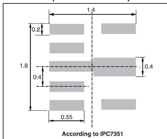
Figure 9. Footprint recommendations (dimensions in mm)
