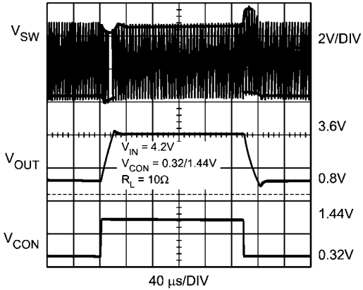
V CON Voltage Response (V IN = 4.2V, V CON = 0.32V/1.44V, R LOAD = 10Ω)
