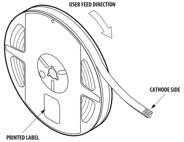
Figure 9. Reeling orientation.
