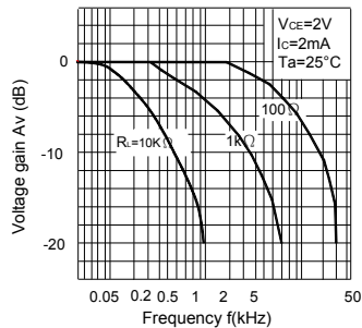
Fig. 10 Frequency Response
