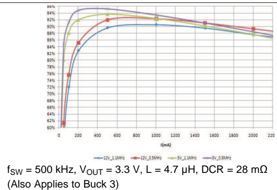
Figure 4. BUCK2 Efficiency
