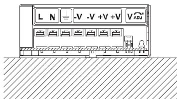
MOUNTING A
