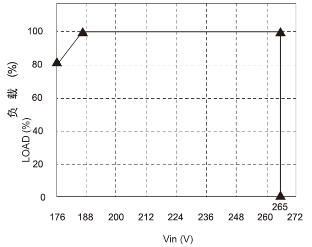
OUTPUT DERATING VS INPUT VOLTAGE
