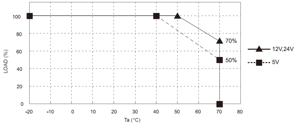
MOUNTING A
