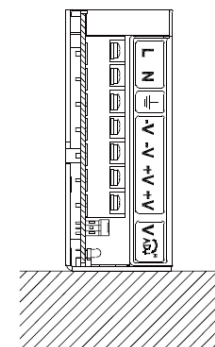
MOUNTING B
