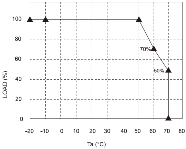
OUTPUT DERATING VS Ta
