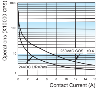
ENDURANCE CURVE(Inductive)
