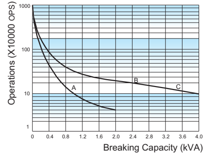
ENDURANCE CURVE(Resistive)
