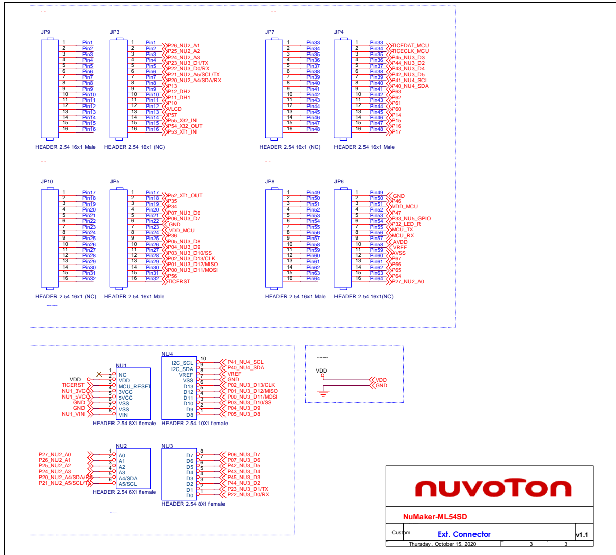
Figure 5-3 Extension Connectors Circuit
