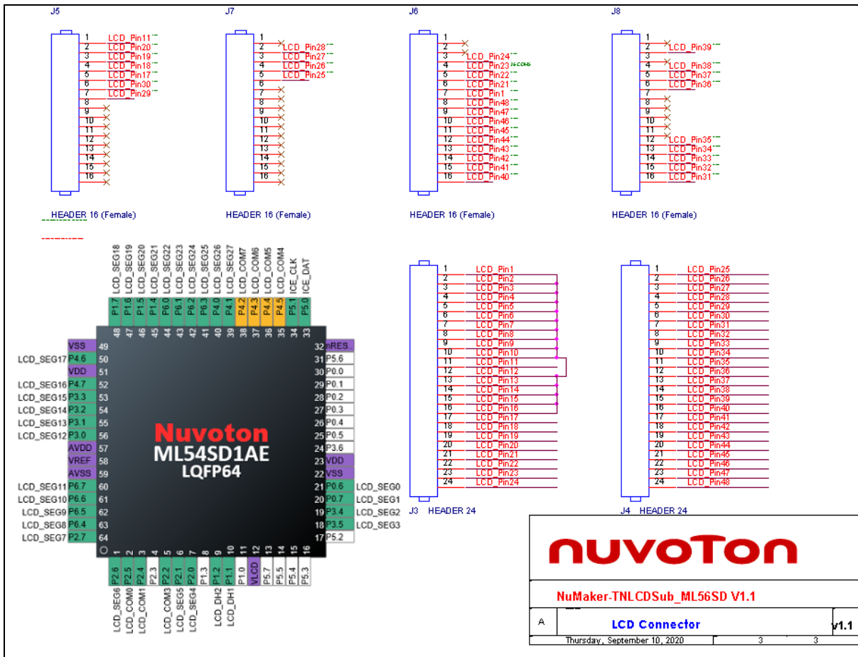
Figure 6-1 LCD Connectors of NuMaker-TNLCDSub_ML56
