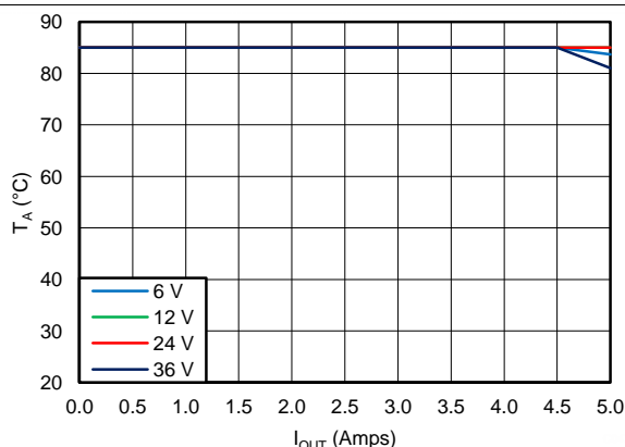
Figure 35. 3.3-V Outputs
