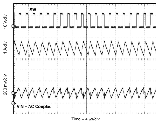
Figure 46. Input Ripple CCM
