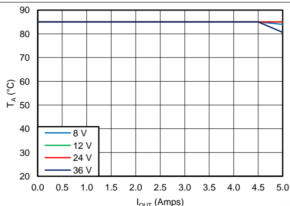
Figure 36. 5-V Outputs
