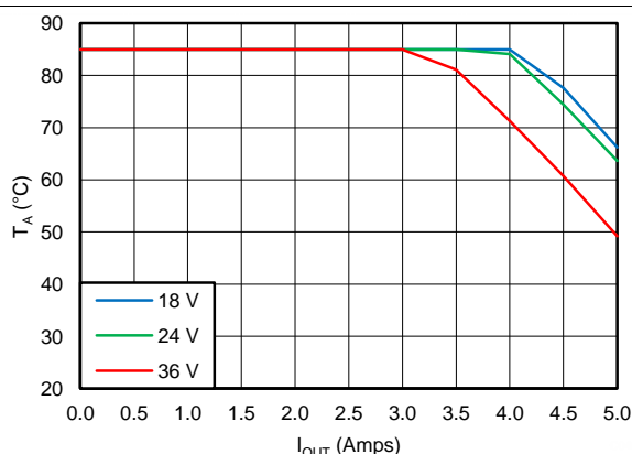
Figure 37. 12-V Outputs
