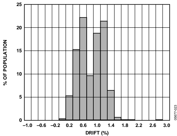
Figure 25. Z-Axis Sensitivity Drift Over Temperature, V_s = 3V
