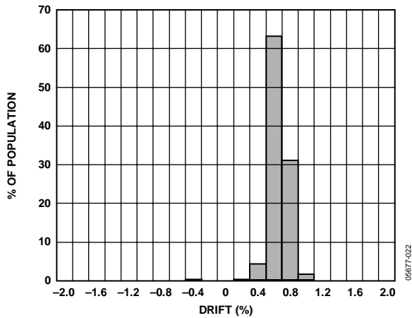
Figure 24. Y-Axis Sensitivity Drift Over Temperature, V_s = 3V
