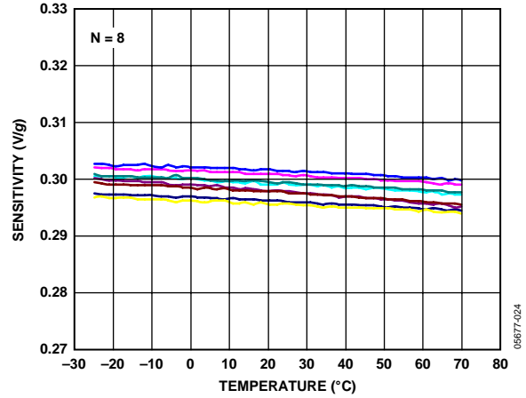
Figure 26. X-Axis Sensitivity vs. Temperature 8 Parts Soldered to PCB, V_s = 3V
