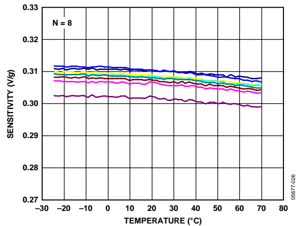
Figure 28. Z-Axis Sensitivity vs. Temperature 8 Parts Soldered to PCB, V_s = 3V
