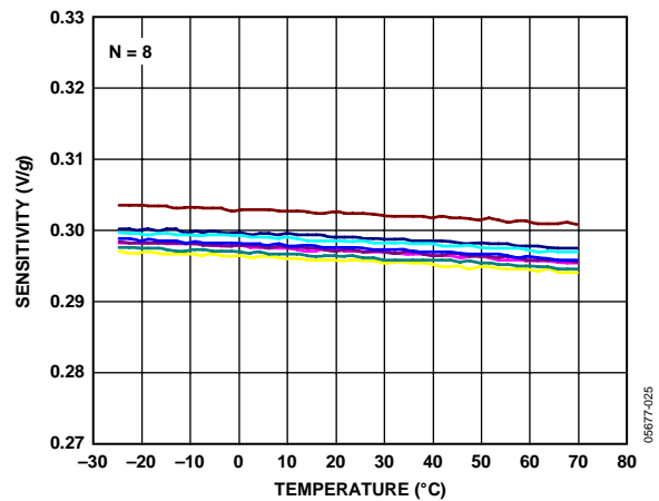
Figure 27. Y-Axis Sensitivity vs. Temperature 8 Parts Soldered to PCB, V_s = 3V
