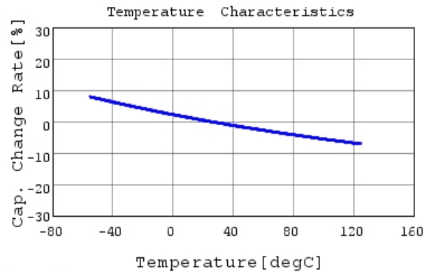
GRM21A7U2E681JW31 C-Temp. capchange, DC0V, f
