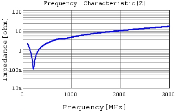
GRM21A7U2E681JW31 |Z| DC0V, 25degC
