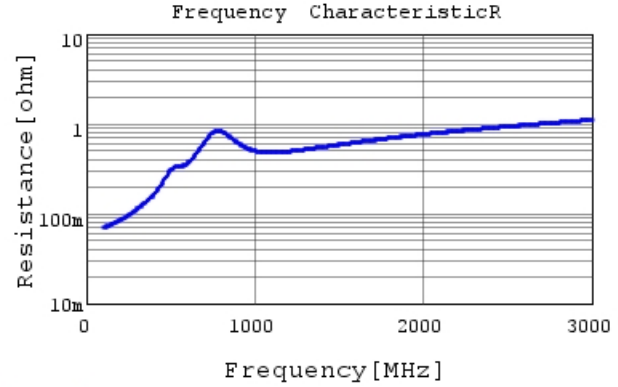
GRM21A7U2E681JW31 R DC0V, 25degC
