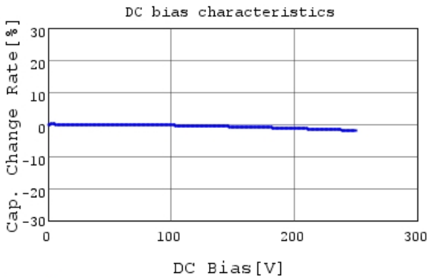
GRM21A7U2E681JW31 C-DC bias capchange, 25.0c
