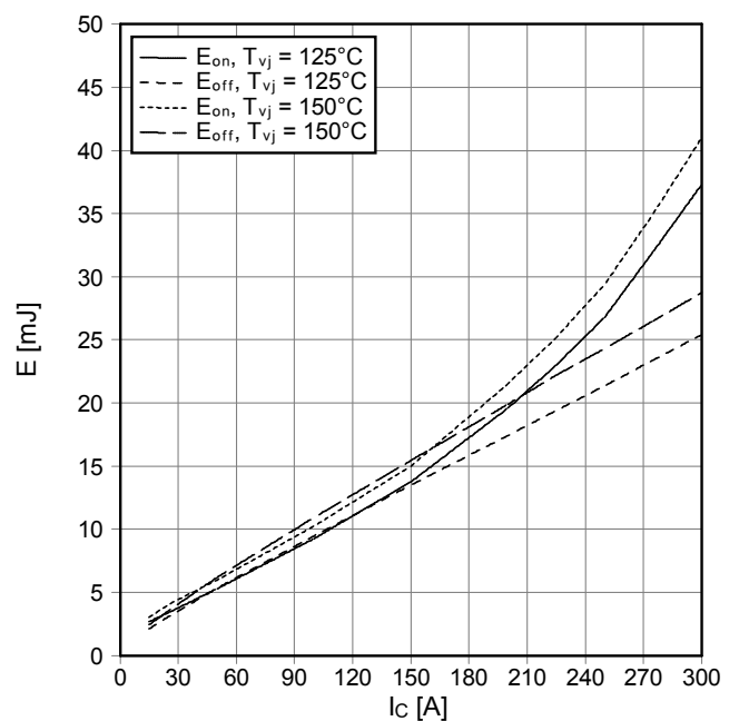
Schaltverluste IGBT-Brems-Chopper switching losses IGBT-brake-chopper E_{on} = f(I_C) , E_{off} = f(I_C) V_{GE} = \pm 15\text{ V} , R_{Gon} = 1.1\ \Omega , R_{Goff} = 1.1\ \Omega , V_{CE} = 600\text{ V}
