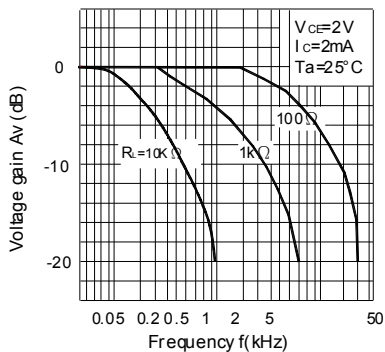
Fig. 10 Frequency Response
