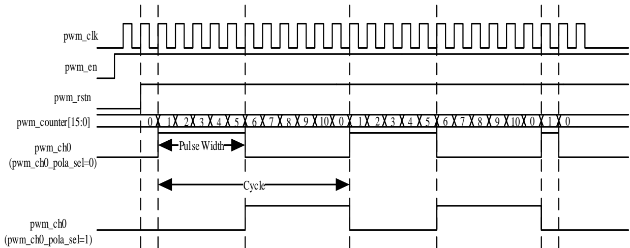
PWM1/2 output waveform
