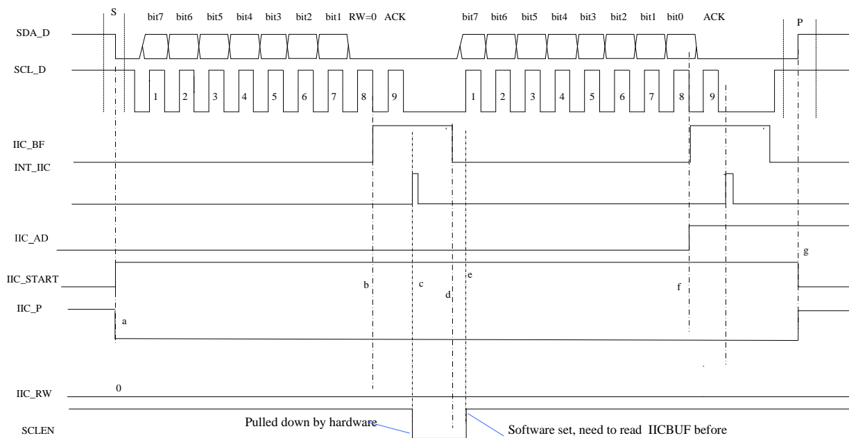
IIC write low clock line diagram
