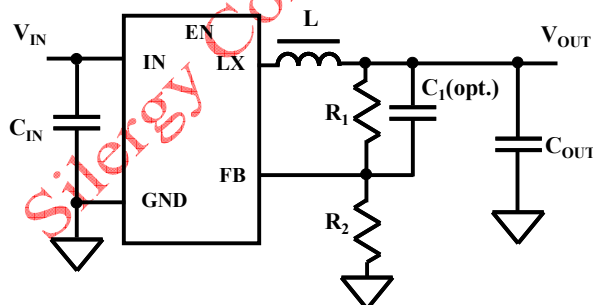
Figure 1. Schematic Diagram
