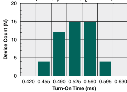
Typical Turn-On Time (N=50, I F =10mA, I L =140mA)
