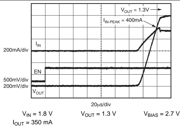
Figure 23. V_{\text{IN}} Inrush Current
