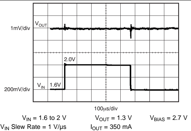
Figure 24. V_{\text{IN}} Line Transient Response
