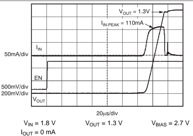
Figure 22. V_{\text{IN}} Inrush Current
