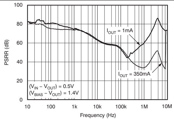
Figure 20. V_{\text{BIAS}} Power-Supply Ripple Rejection vs Frequency (TPS72015YZU)
