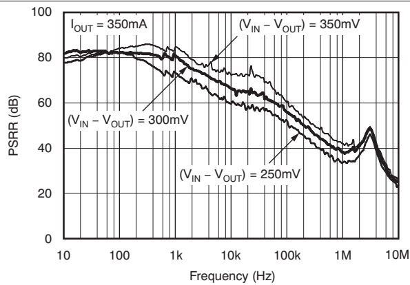
Figure 19. V_{\text{IN}} Power-Supply Ripple Rejection vs Frequency (TPS72015YZU)
