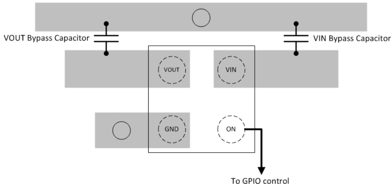
Figure 32. Layout Example
