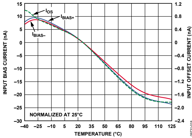
Figure 16. Input Bias Current and Input Offset Current vs. Temperature, Normalized at 25°C
