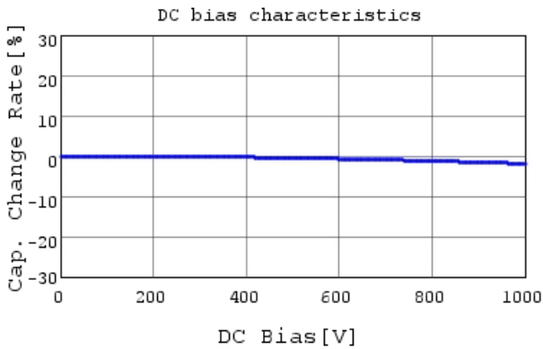
GRM31B7U3A471JW31 C-DC bias capchange, 25.0c
