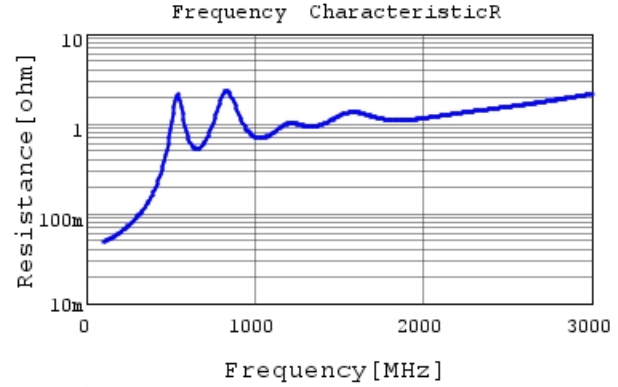
GRM31B7U3A471JW31 R DC0V, 25degC
