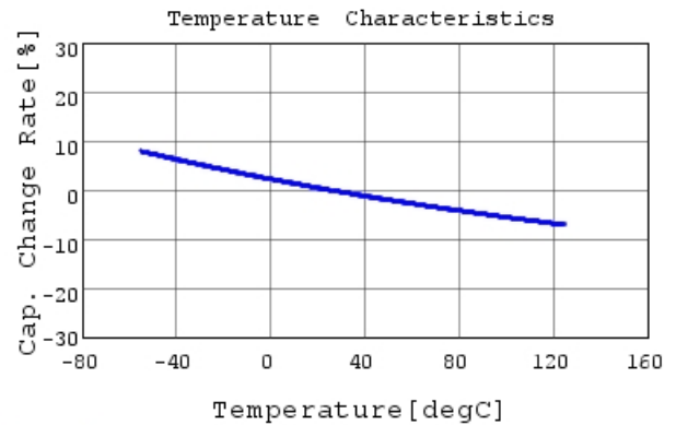
GRM31B7U3A471JW31 C-Temp. capchange, DC0V, 1
