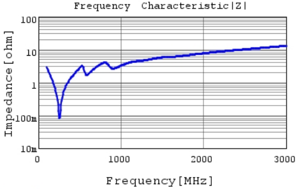
GRM31B7U3A471JW31 |Z| DC0V, 25degC
