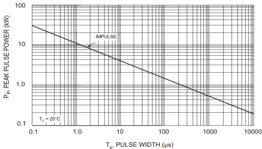
Fig. 3 Pulse Rating Curve
