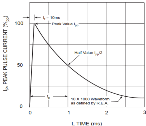
Fig. 1 Pulse Waveform
