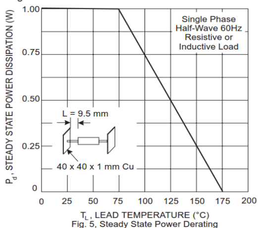
Fig. 5, Steady State Power Derating
