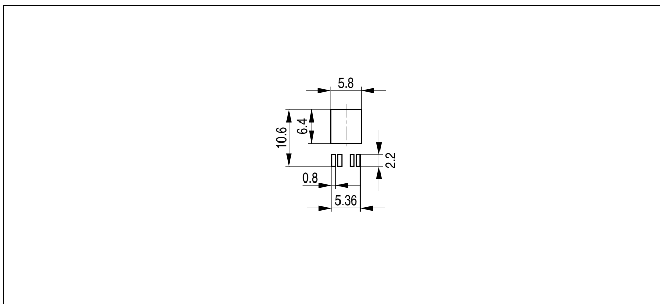
Figure 5 Foot Print for PG-TO-252-5-11 (Plastic Transistor Single Outline)
