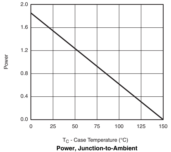
Power, Junction-to-Ambient
