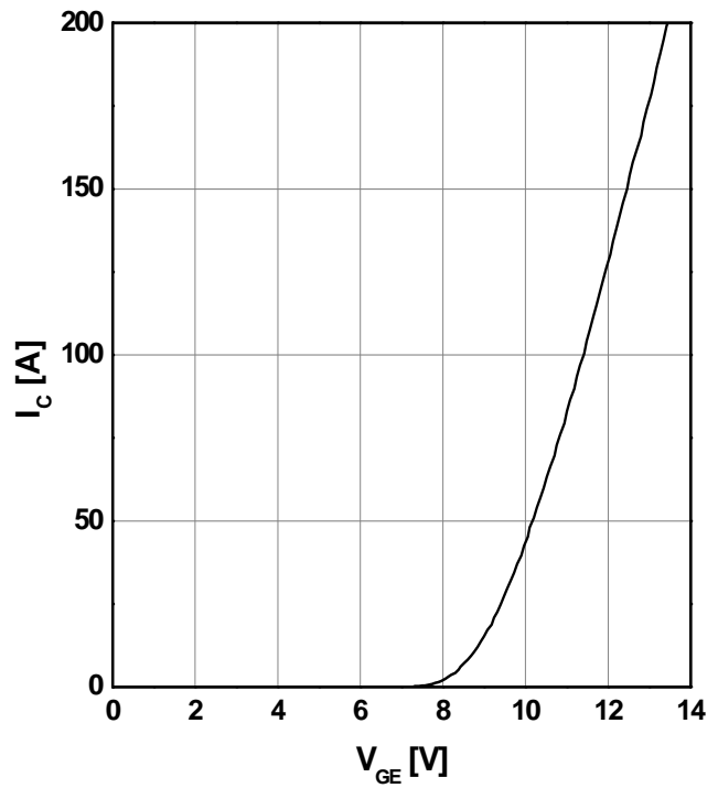
Fig2. Transfer Characteristics
