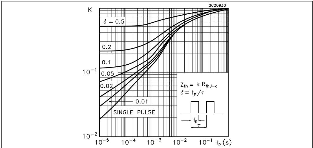
Figure 27. thermal impedance for diode
