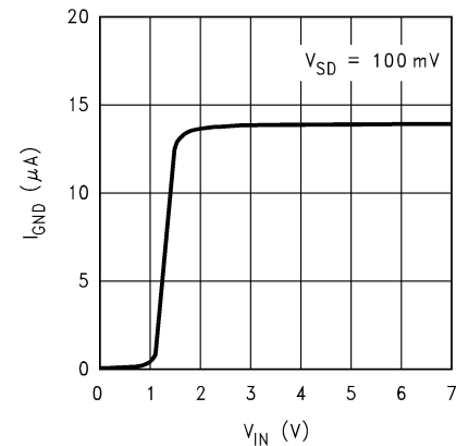
Ground Pin Current Vs Input Voltage ( V_{SD}=100mV )
