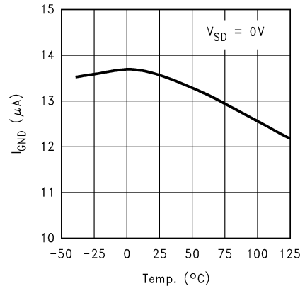
Ground Current Vs Temperature ( V_{SD}=0V )
