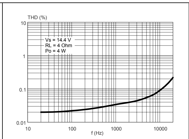
Figure 9. Distortion vs. frequency (4 \Omega )
