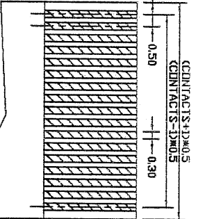
FFC/FPC DIMENSION THICKNESS 0.30 mm
