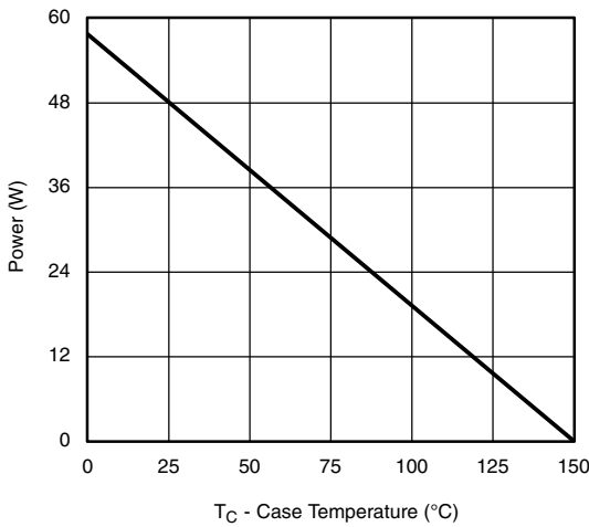
Power, Junction-to-Case
