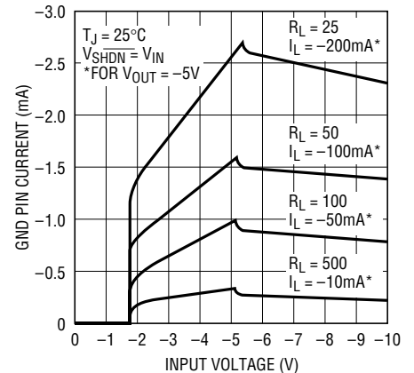
LT1964-5 GND Pin Current
