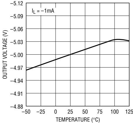
LT1964-5 Output Voltage
