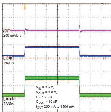
Figure 19. Load Transient Response 200 mA to 1500 mA
