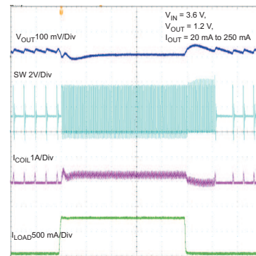
Figure 18. Load Transient PFM Mode 20 mA to 250 mA
