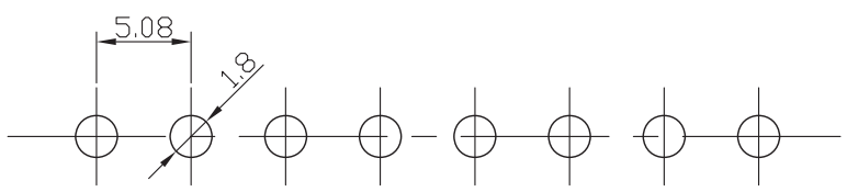
RECOMMENDED P.C. BOARD HOLE DIM.
