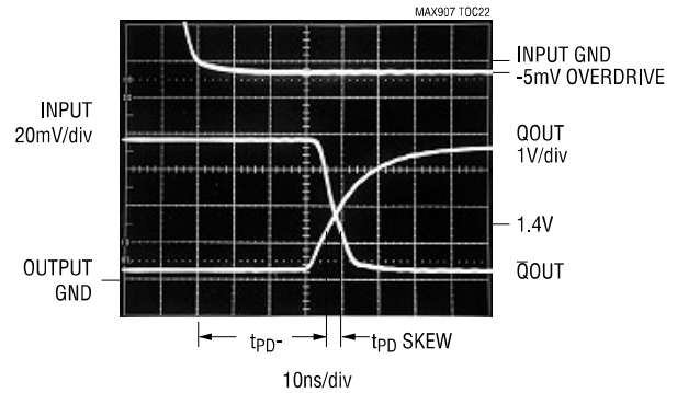
MAX909 PROPAGATION DELAY (t PD- ) (5mV OVERDRIVE)
