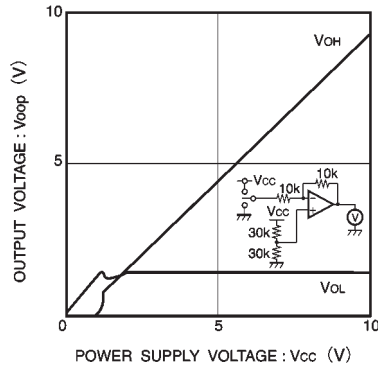
Fig. 7 Power supply voltage vs. operational amplifier high / low level output voltage
