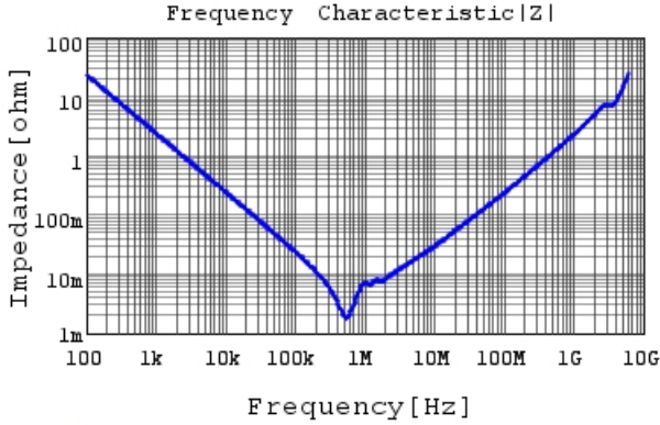
GRM32EC70J107ME15 |Z| DCOV,25degC
