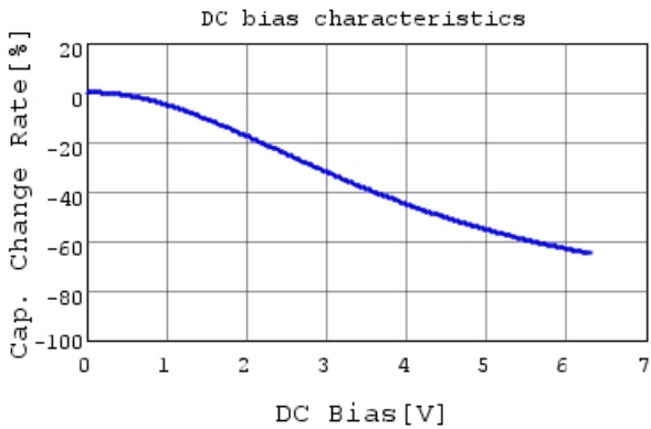
GRM32EC70J107ME15 C-DC bias capchange, 25.0c
