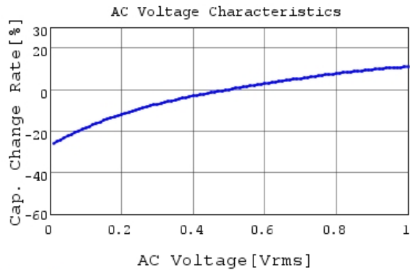
GRM32EC70J107ME15 C-AC Voltage capchange, Dc
