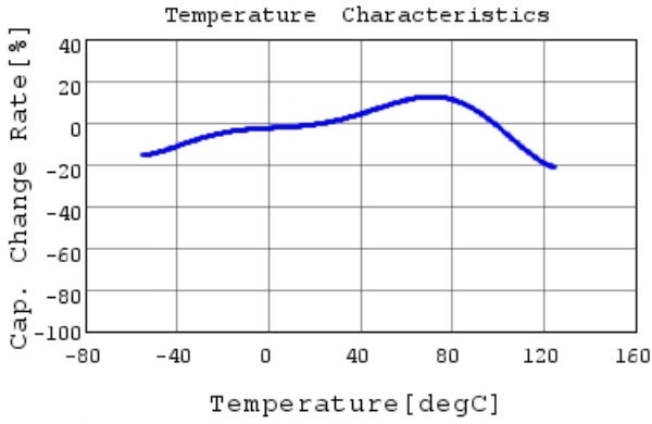
GRM32EC70J107ME15 C-Temp. capchange, DC0.0V,
