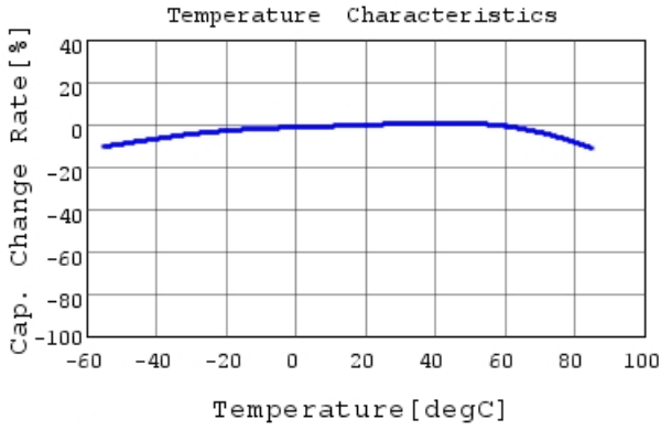
GRM033R61A224ME90 C-Temp. capchange, DC0.0V,
