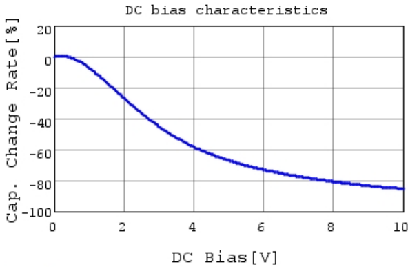
GRM033R61A224ME90 C-DC bias capchange, 25.0c
