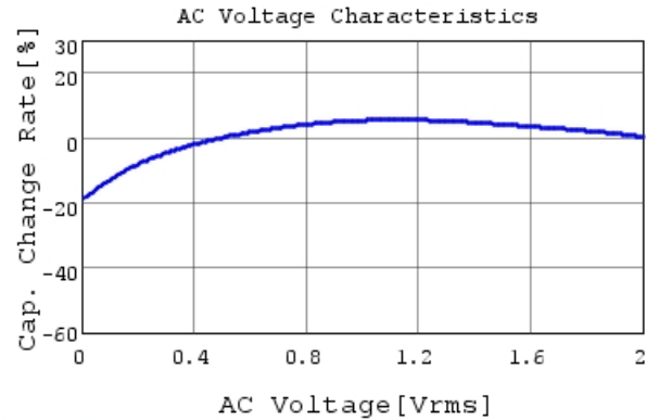
GRM033R61A224ME90 C-AC Voltage capchange, Dc
