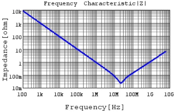
GRM033R61A224ME90 |Z| DCOV, 25degC
