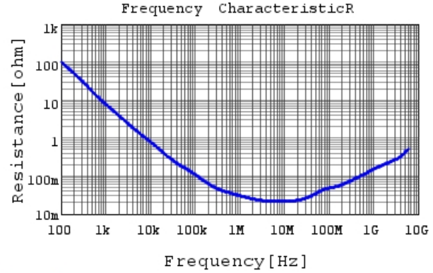
GRM033R61A224ME90 R DCOV, 25degC
