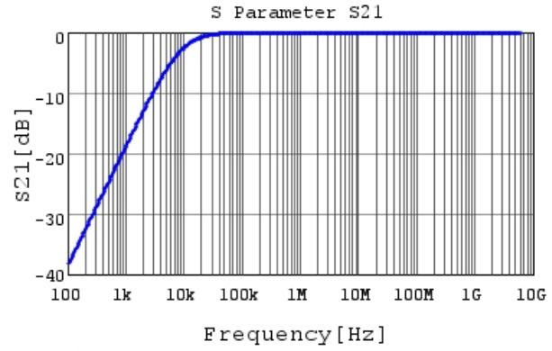
GRM033R61A224ME90 S21 DC0V, 25degC
