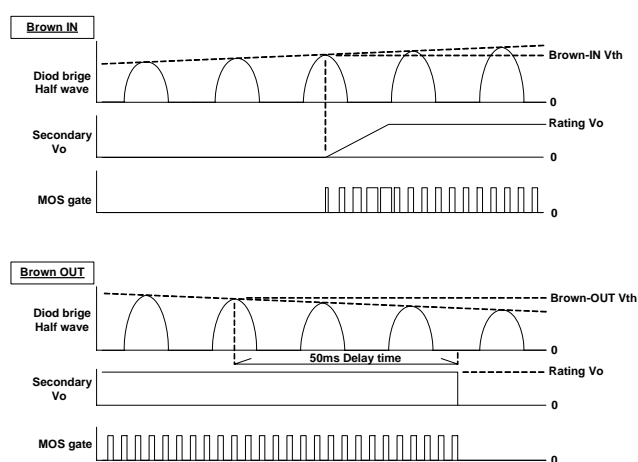
Fig. 20 Conceptual diagram of brown in and brown out operations
