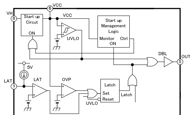
Fig. 18 Overvoltage protection circuit
