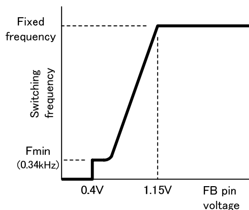
Fig. 4 Oscillation frequency
