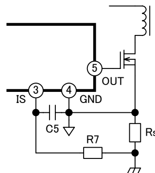
Fig. 30 IS terminal filter
