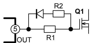
Fig. 27 Gate drive circuit (2)
