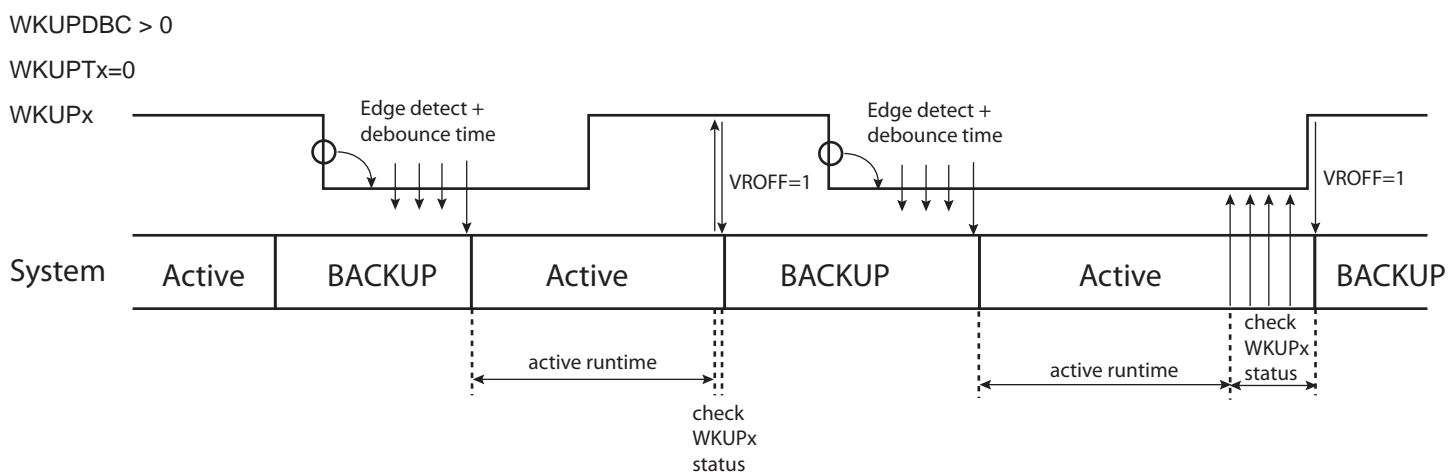
Figure 25-5. Entering and Exiting Backup Mode with a WKUP pin
