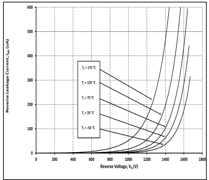
Figure 2. Reverse Characteristics
