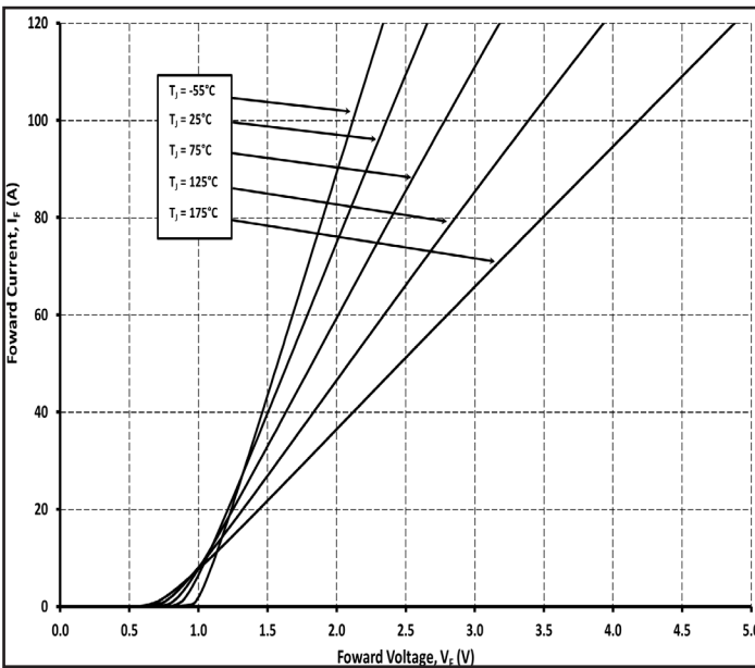
Figure 1. Forward Characteristics
