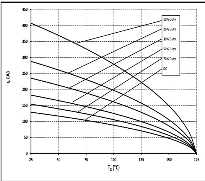
Figure 3. Current Derating
