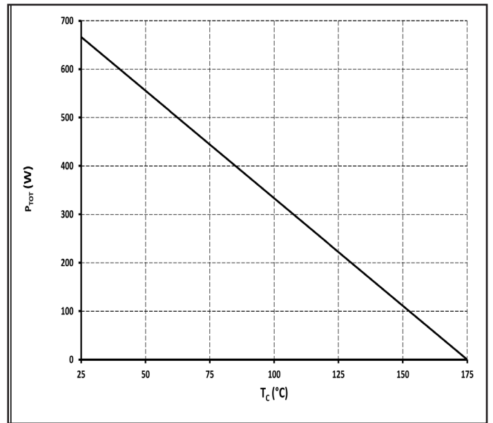
Figure 4. Power Derating
